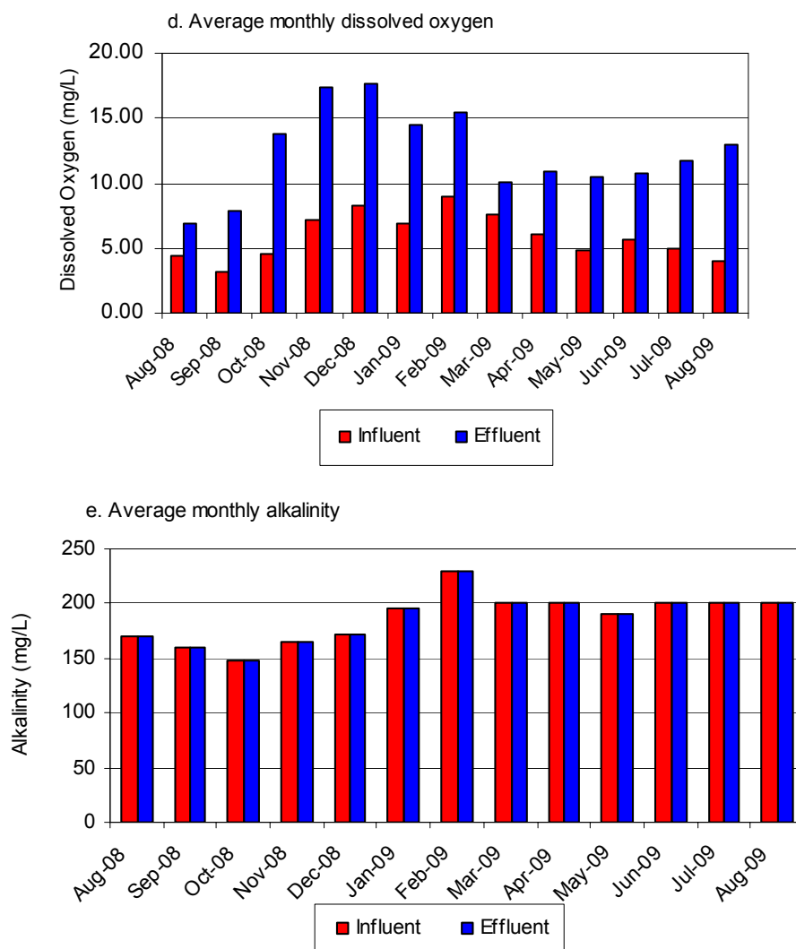
Figure 16 (Cont). Mean monthly ambient water quality parameters at the STA-1W ATS™ Pilot (a through e) based upon daytime sampling.
