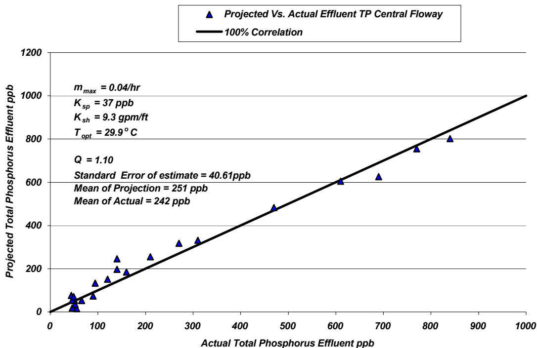
Figure A2-11: Actual Vs. ATSDM Projected total phosphorus effluent concentration Central Floway
