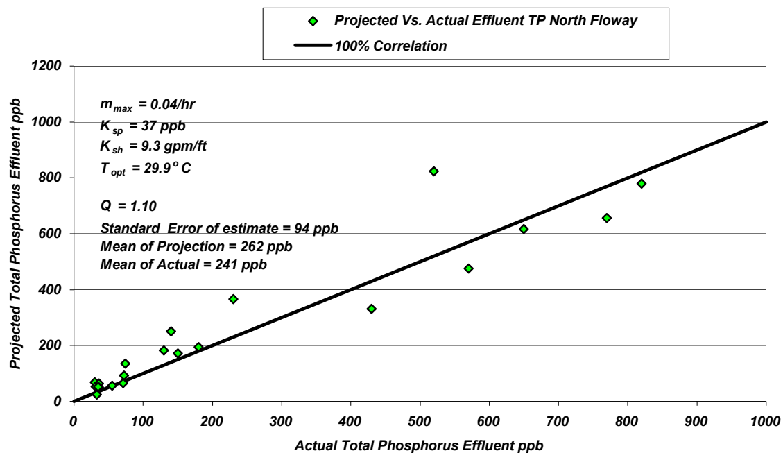
Figure A2-12: Actual Vs. ATSDem Projected total phosphorus effluent concentration North Flowway
