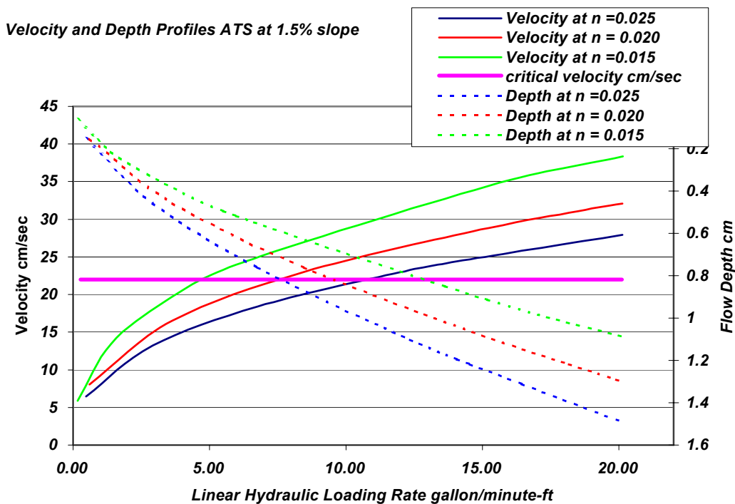
Figure A2-14: Velocity, LHLR and depth relationships as determined from Manning Equation
