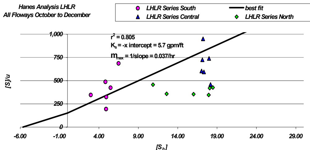
Figure A2-10: Hanes plot LHLR all floways October to December
