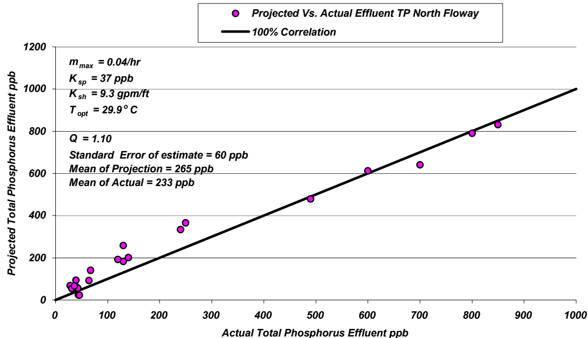
Figure A2-13: Actual Vs. ATSDem Projected total phosphorus effluent concentration South Flowway
